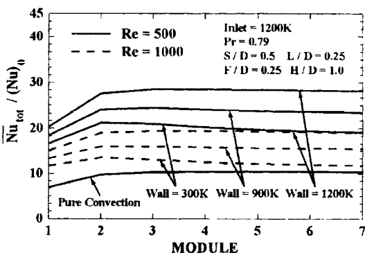
Fig. 10 Total Nusselt number variation for the Reynolds number
