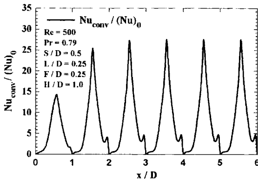
Fig. 7 Local convection Nusselt number variation
