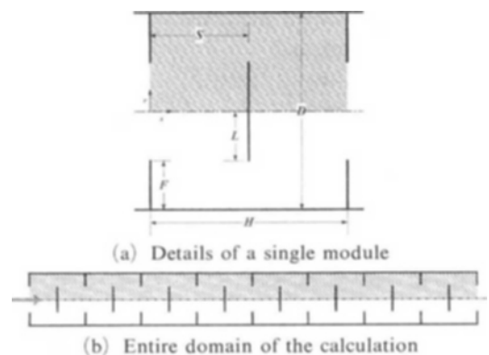
Fig. 1 Considered disk and doughnut geometry
